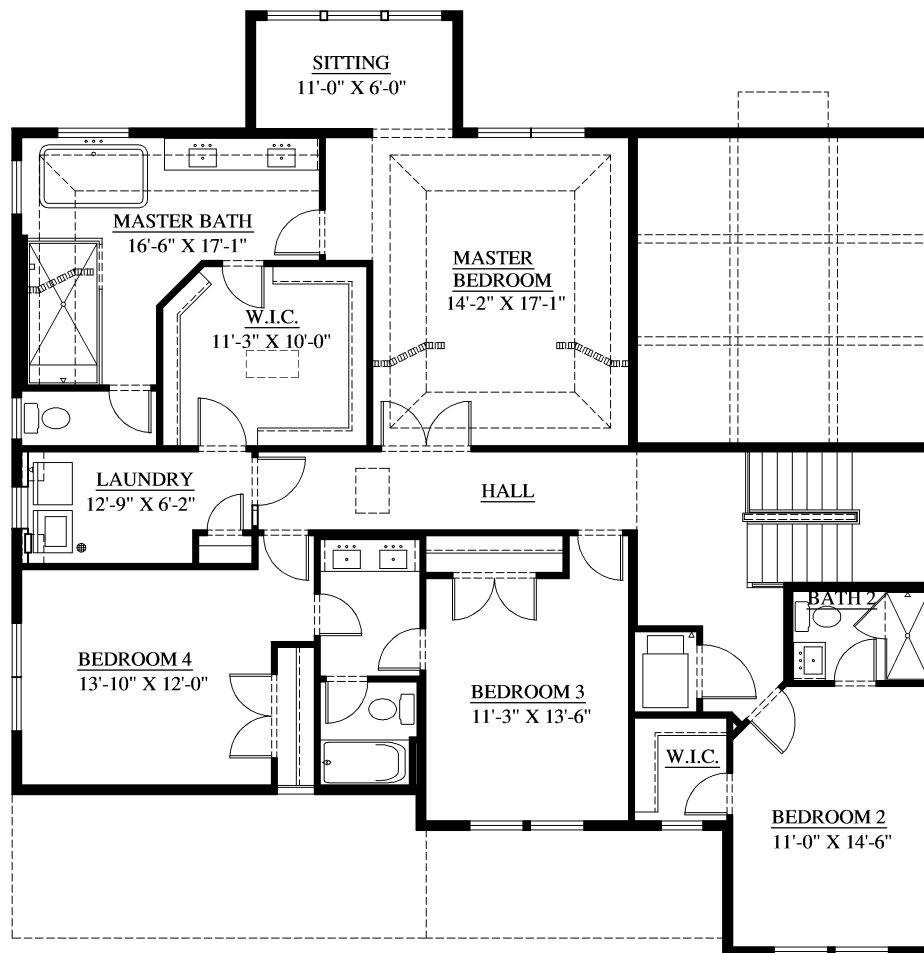
SECOND FLOOR 2126 S.F.
