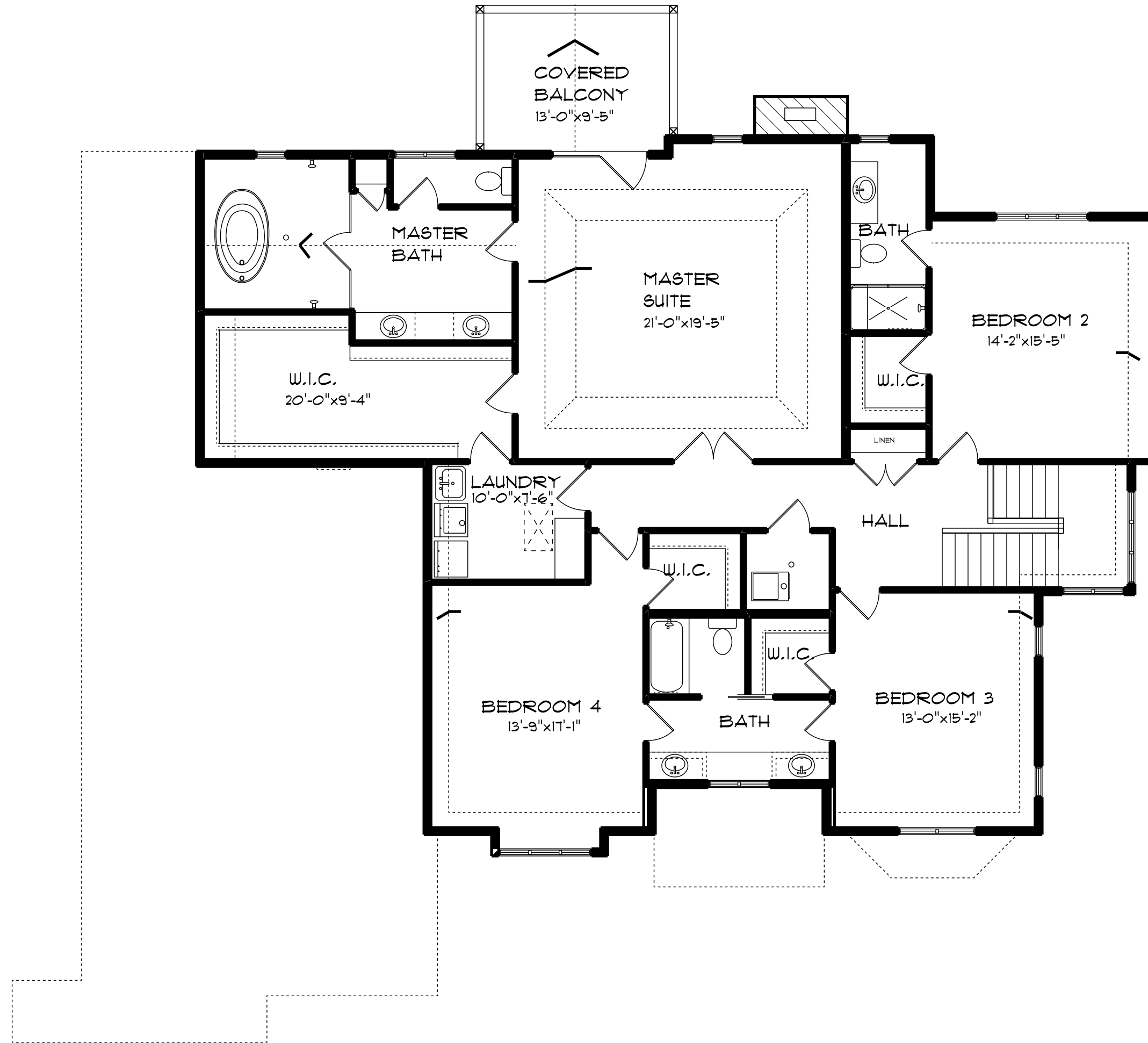
SECOND FLOOR
