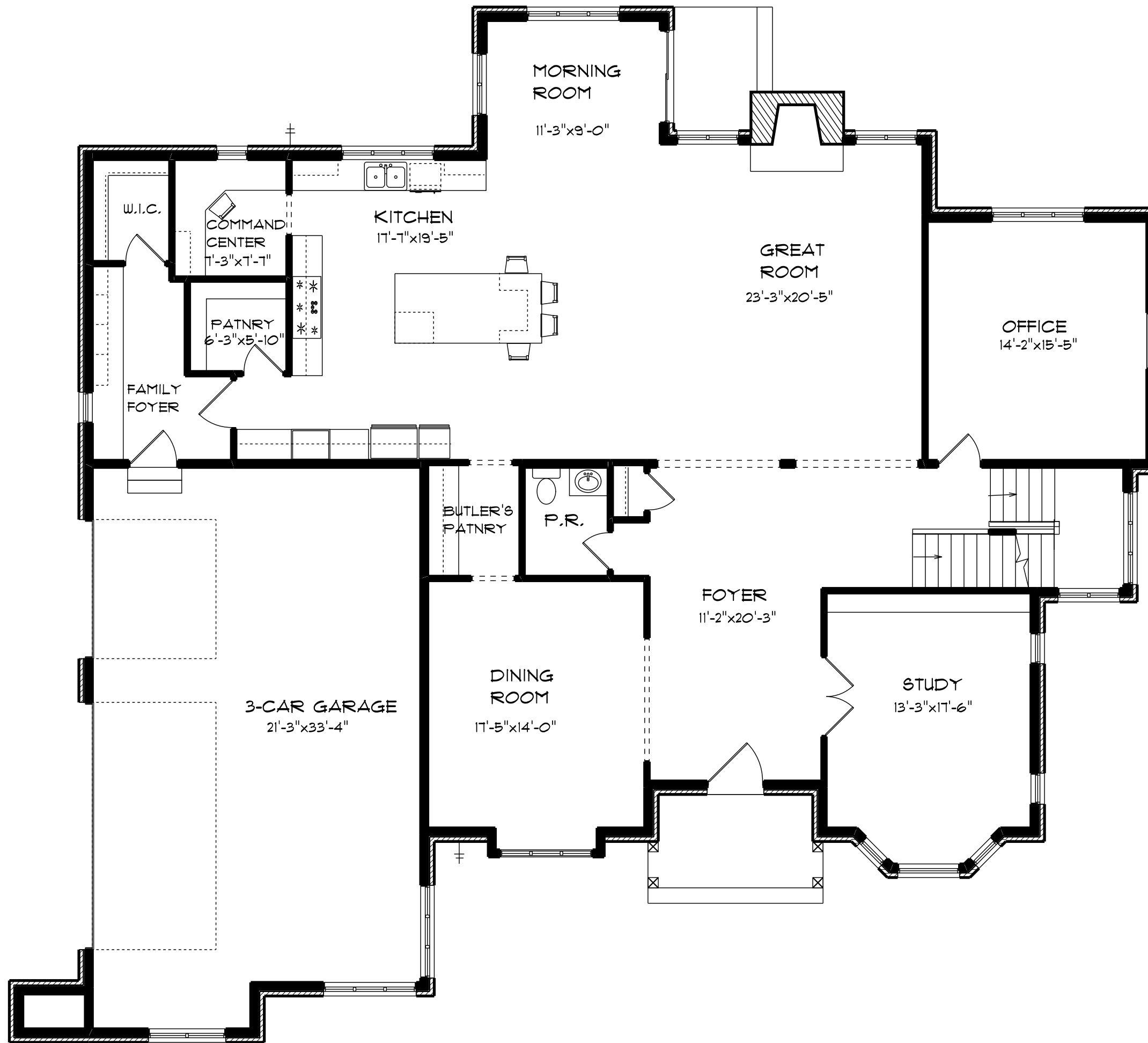
FIRST FLOOR
