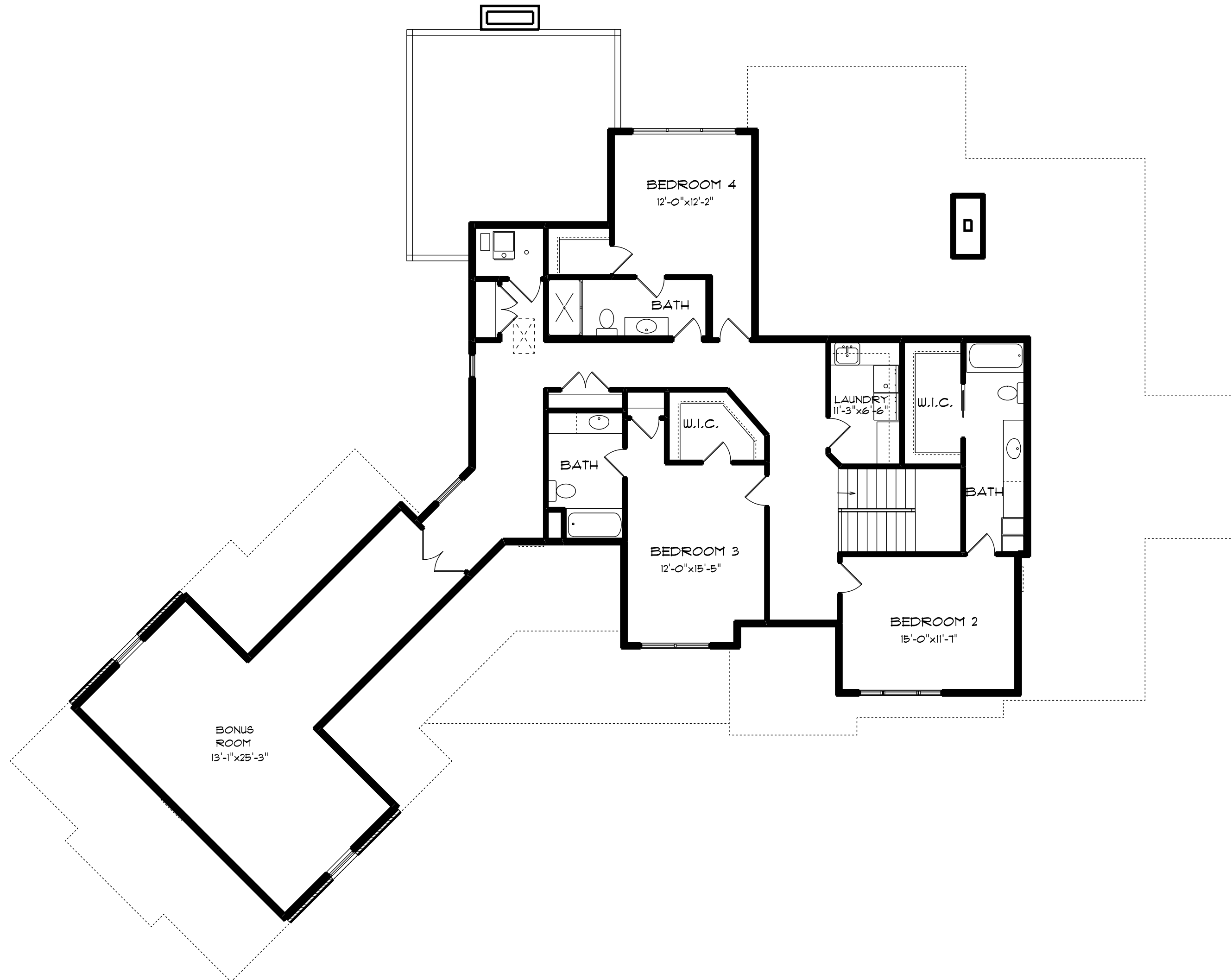
SECOND FLOOR PLAN LOT 5
