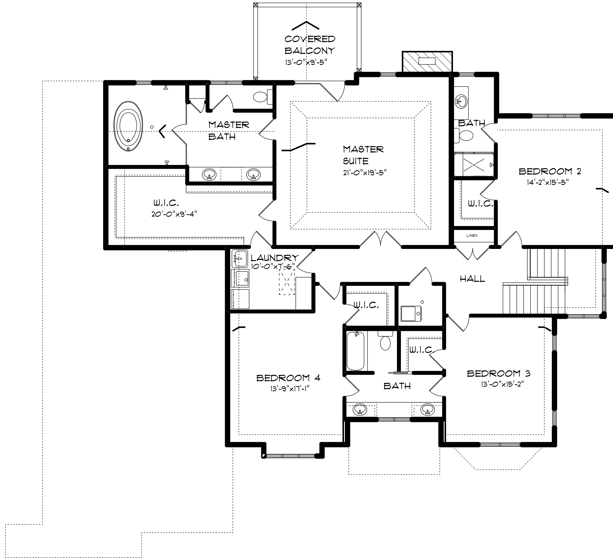
SECOND FLOOR
