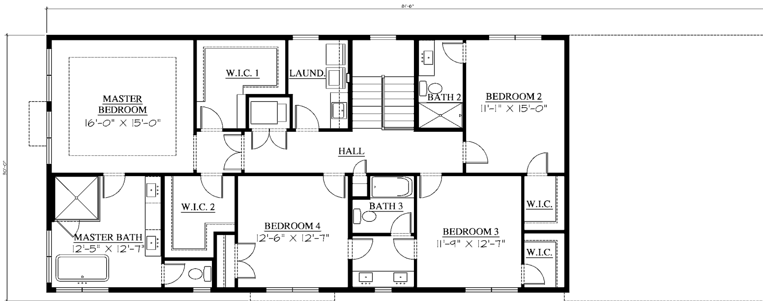
SECOND FLOOR 1,711 S.F.
